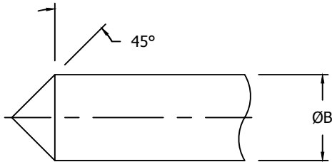
FIGURE 5 - INTERNAL FLARING TOOL
